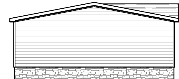
LEFT ELEVATION
